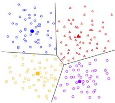
Figure 4-Clustering Model
