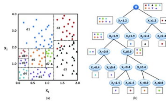
Figure 3-Decision tree model
